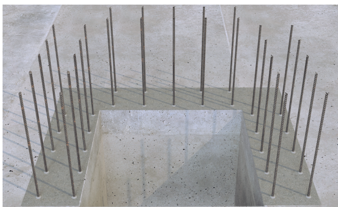
Post-installed rebar connections
